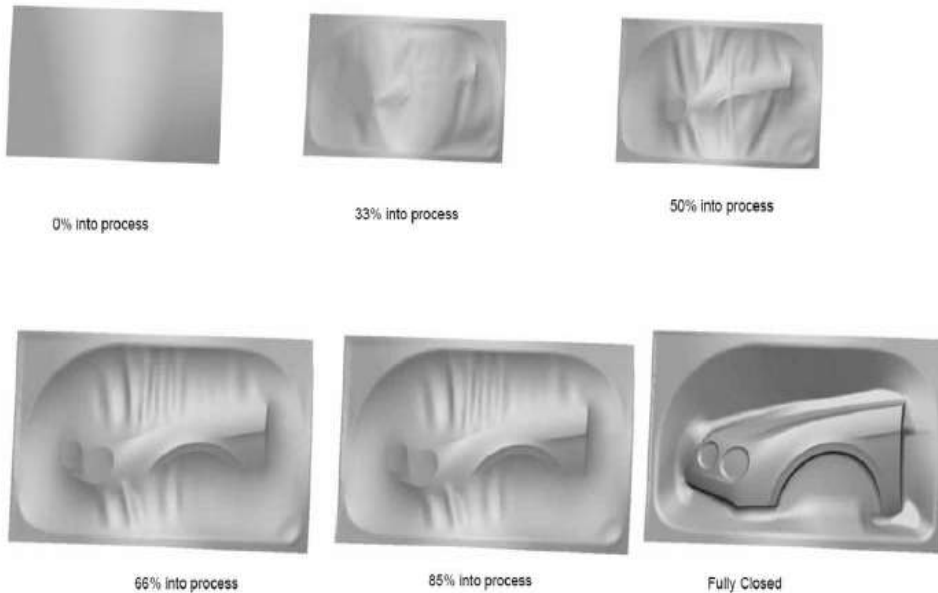
Simulation of SPF Forming process
