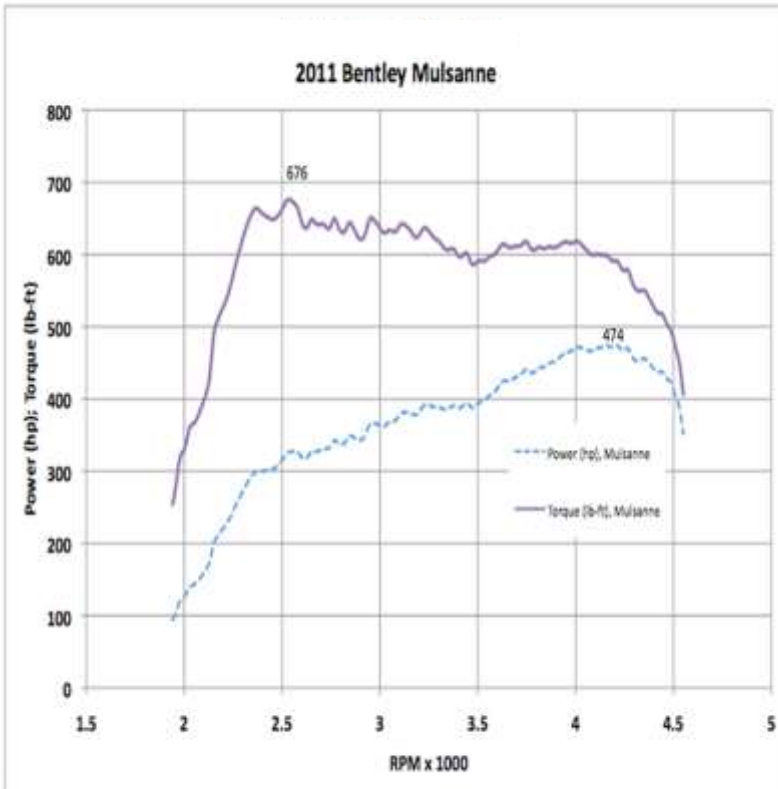
Mulsanne Torque Graph
